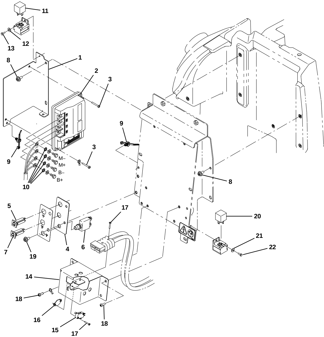
Fig. 26 – Electrical Group
