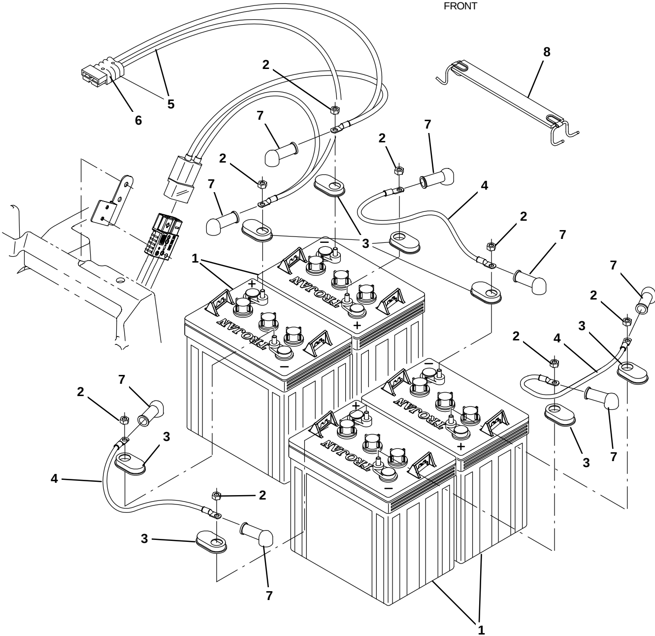
Fig. 5 – Battery Group, 210AH, C20
