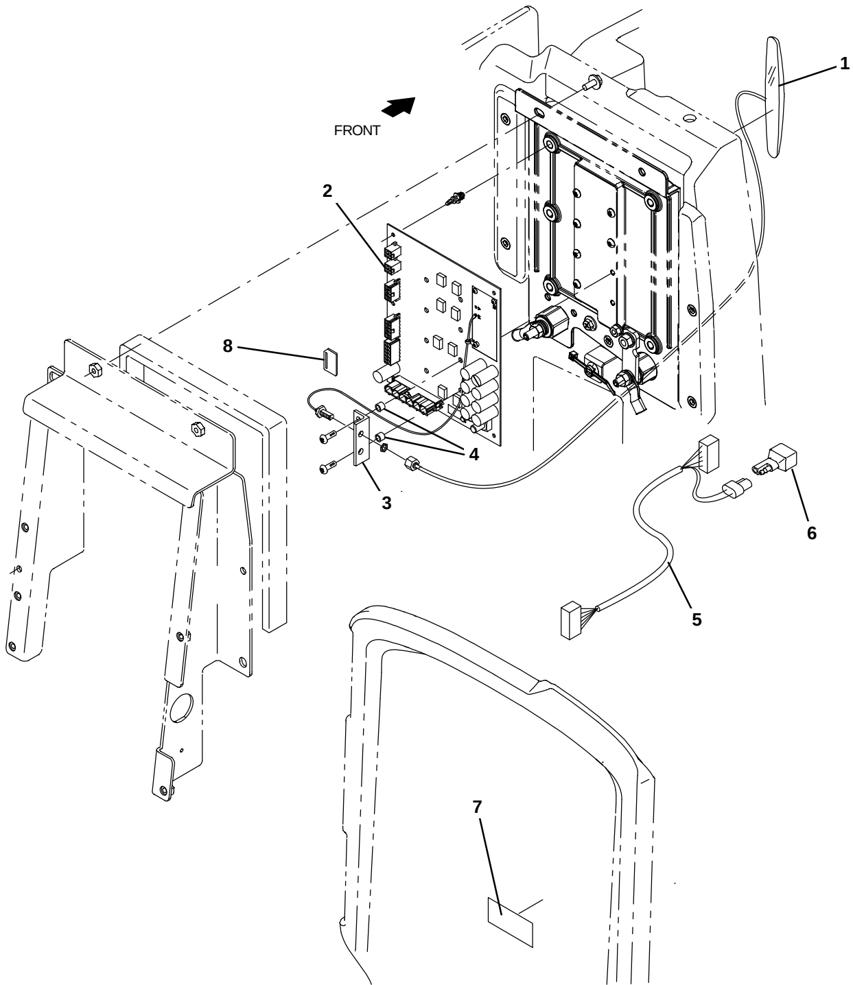
Fig. 4 – Telemetry Group
